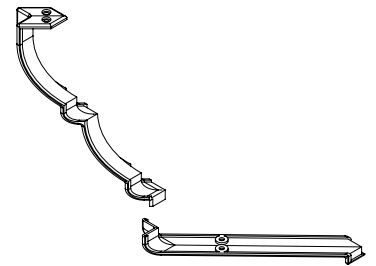
Internal 90° corner casting CRS 8573A
